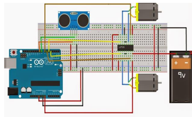
Fig -2:Block diagram of obstacle sensing robot process
