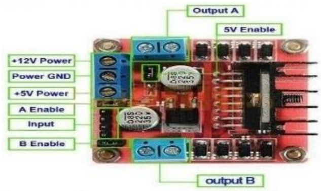
Fig -6: Motor drive module diagram
