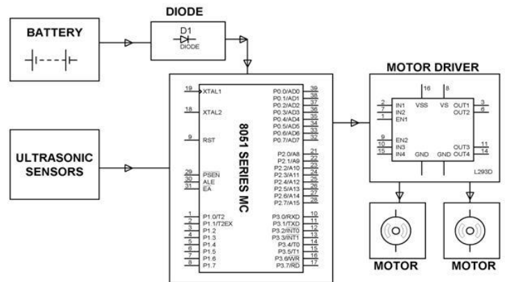
Fig -5: Circuit diagram for ultrasonic sensor and controller using Arduino controller
