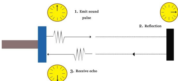
Fig -4:Timing Diagram
