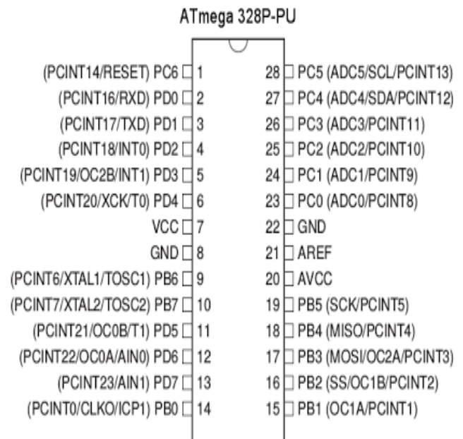
Fig -7: Pin configuration of atmega328P-PU microcontroller
