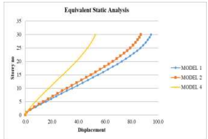
Fig. 3 Comparison of story v/s displacement for 30 storey different models in x-direction
