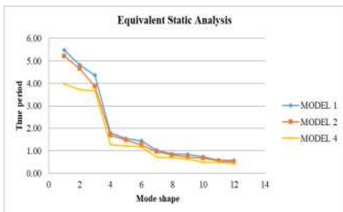
Fig. 7 Comparison of mode numbers v/s time period for 30 storey different models
