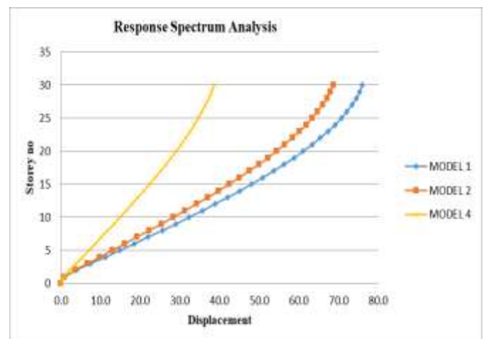
Fig. 4 Comparison of story v/s displacement for 30 storey different models in x-direction
