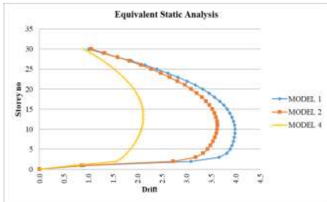
Fig. 5 Comparison of storey v/s storey drifts for 30 story different models in x-direction
