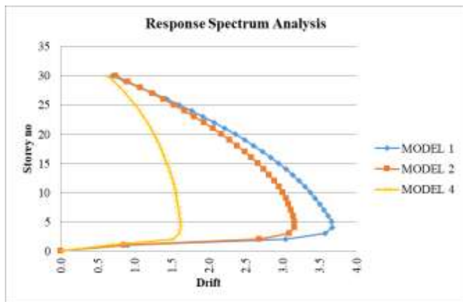
Fig. 6 Comparison of storey v/s storey drifts for 30 story different models in x-direction
