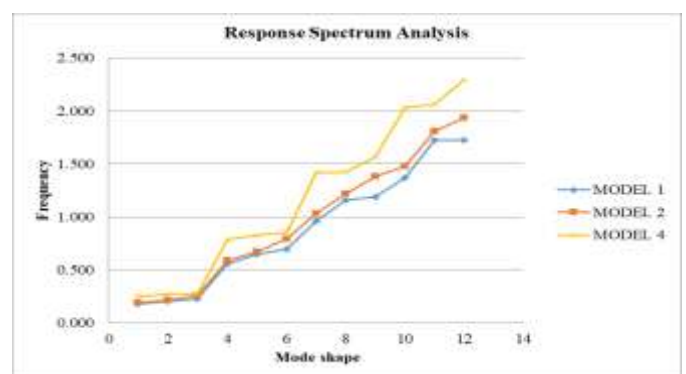
Fig.10 Comparison of mode numbers v/s frequency for 30 storey different models
