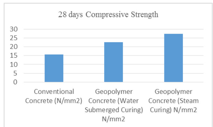
Figure 3: 28 days Compressive Strength
