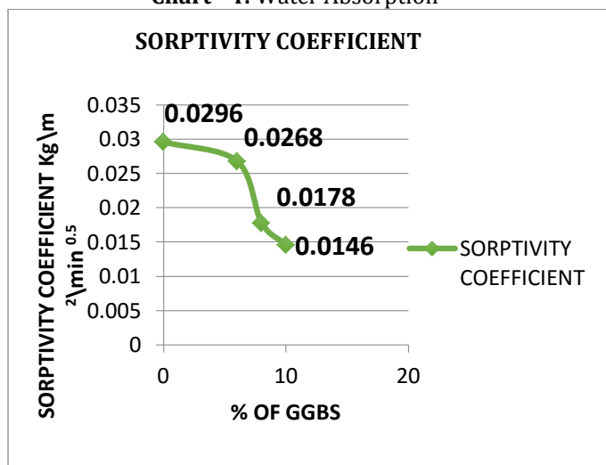
Chart - 4: Water Absorption
