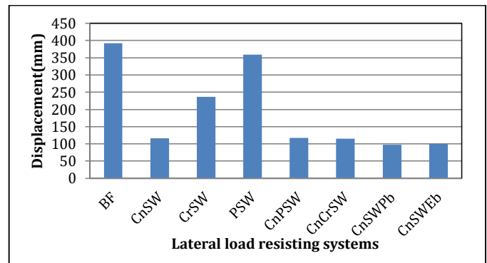
Chart 1: Storey displacement V/s LLRS
