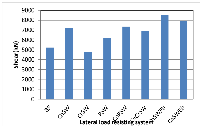
Chart 7: Base shear in Y direction V/s LLRS
