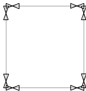
Fig 3: Position of bracings in flat slab building with CnSWEb
