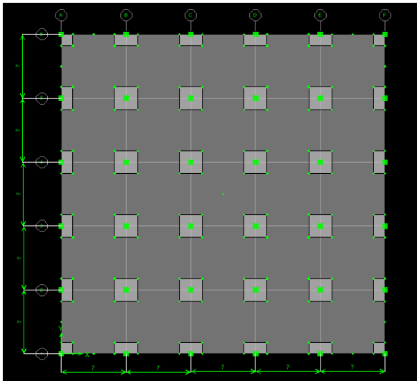
Fig. 1: Plan of the RC flat slab building
