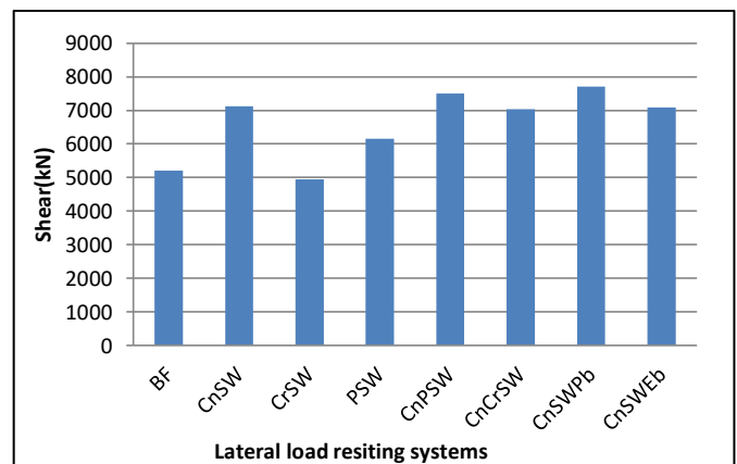
Chart 6: Base shear in X direction V/s LLRS
