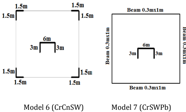
Fig-2: Plan of various models used
