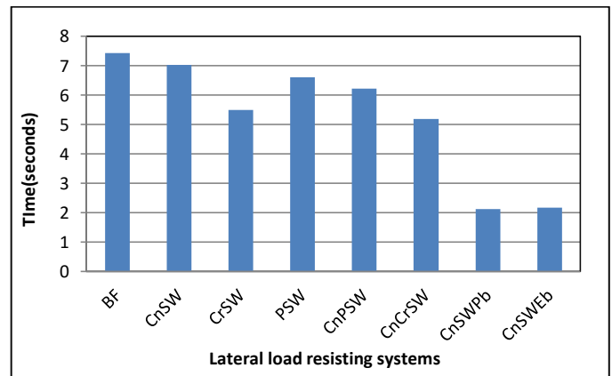
Chart 5: Time period V/s LLRS
