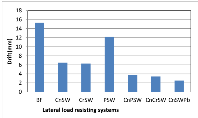
Chart 3: Storey drift V/s LLRS
