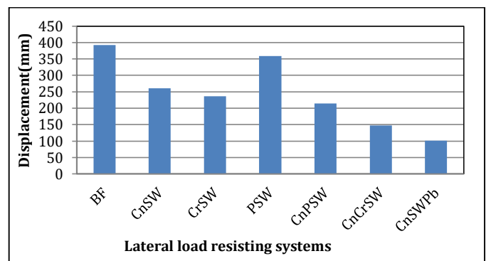
Chart 2: Storey displacement V/s LLRS
