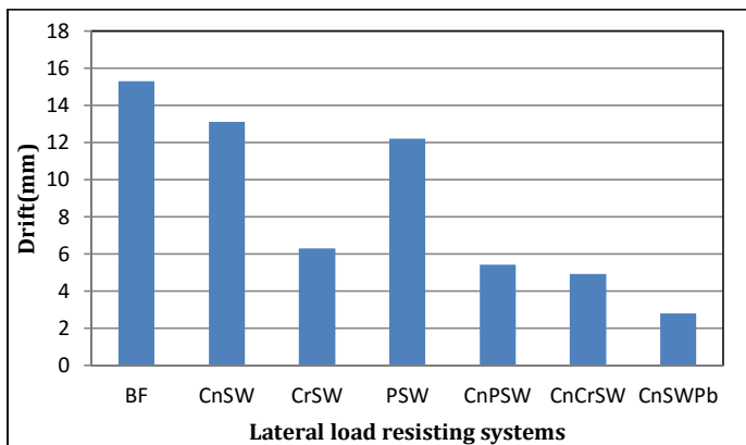
Chart 4: Storey drift V/s LLRS
