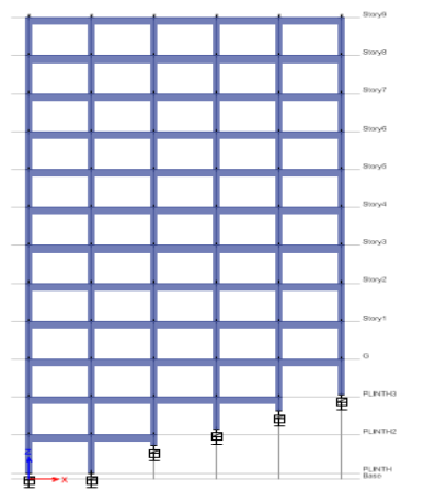
Fig10:20° Slope for lead rubber
