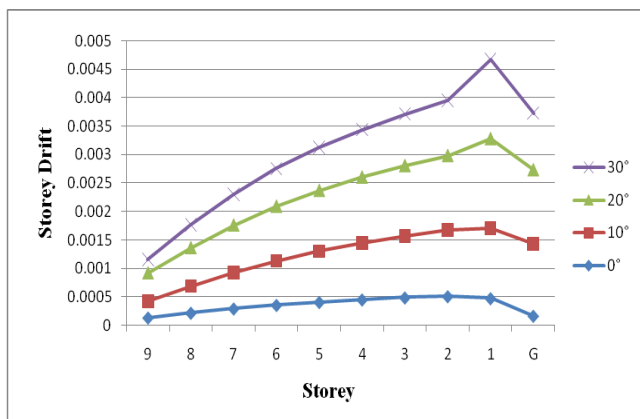
Fig12: Storey drifts in y-direction
