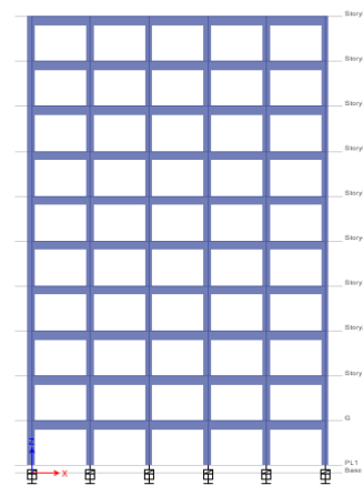
Fig8: 10° Slope for lead rubber
