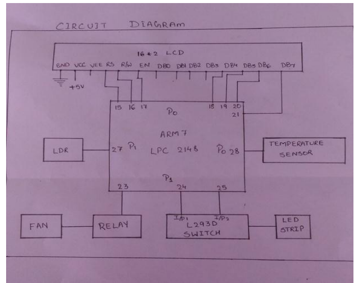
Fig 3: Circuit Diagram
