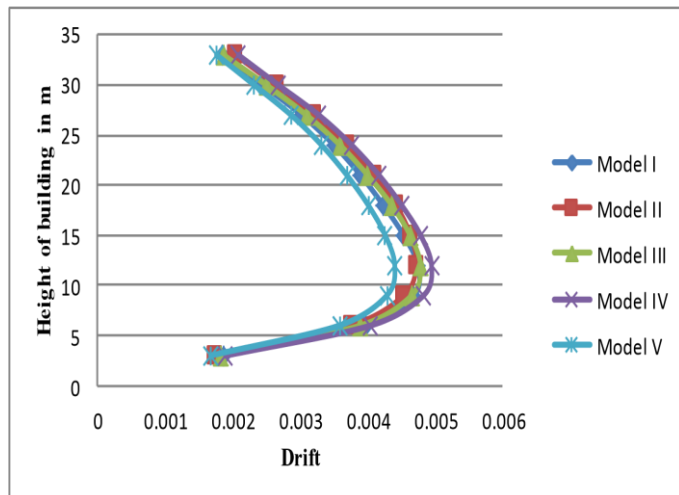
Figure 6. Storey Drift in X-Direction
