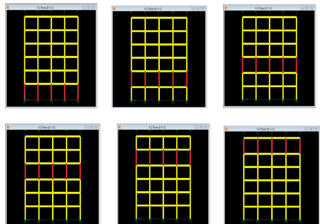
Fig. 1 Model SI1 to SI6
