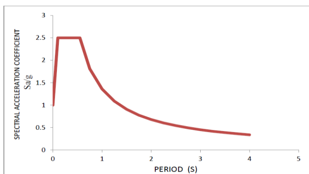
Fig 2: Response Spectra for 5% Damping (IS1893:2002)
