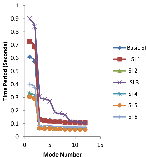
Fig 3: Comparative Graphs for Time Period of Vibrations for Stiffness Irregularity for Various Models
