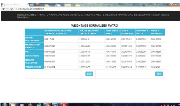
Fig -7: Weightage normalized matrix
