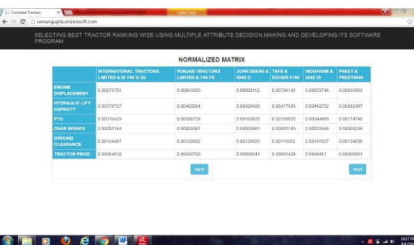
Fig -6: Normalized matrix
