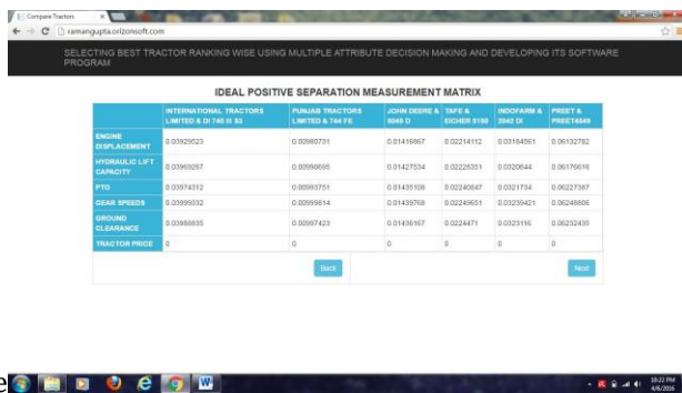
Fig -8: Ideal positive measurement matrix
