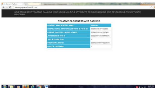
Fig -10: Relative closeness and ranking
