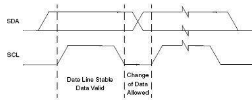
Figure 3: Data Validity
