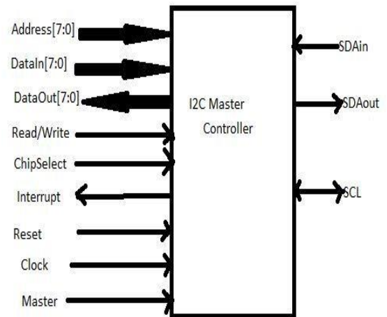
Figure: Symbol of I2C Master Controller
