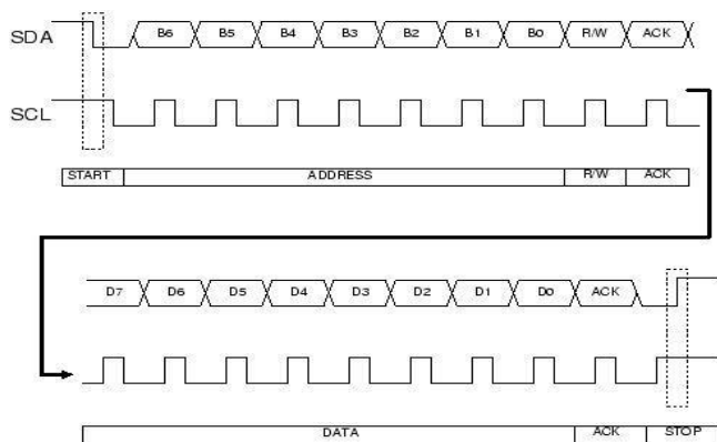
Figure 7: Frame format
