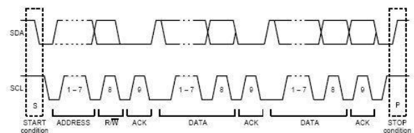
Figure 4: Byte-wise transfer
