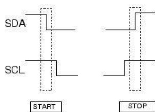
Figure 2: Start and Stop Conditions on C Bus
