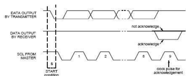
Figure 6: Acknowledge on C Bus
