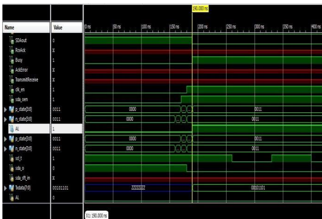
10: Simulation Waveform for Multi – Master I2C Bus Controller
