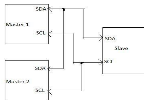
Figure 1: Multi – Master C devices
