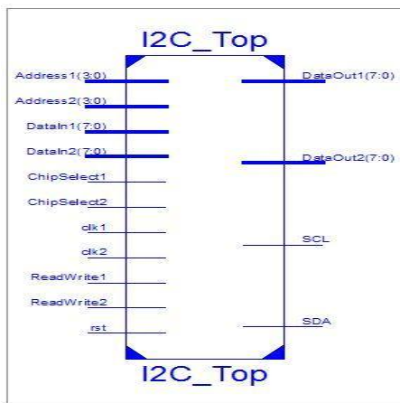
Figure 11: RTL View
