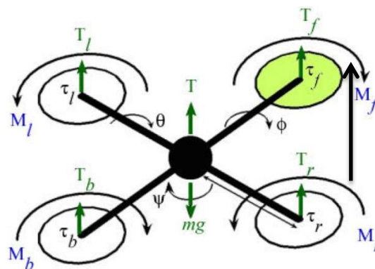
Fig.2 VTOL of quad copter [7]
