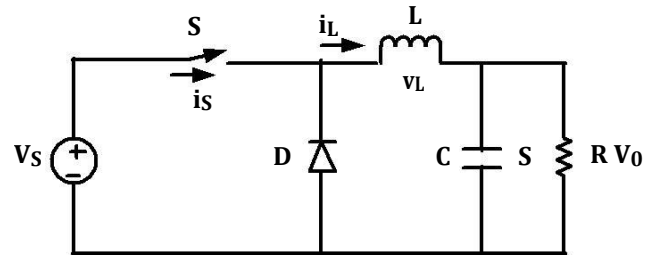
Fig. 4. Buck Converter
