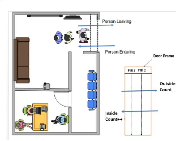
Fig. 7. Visitors Counter
