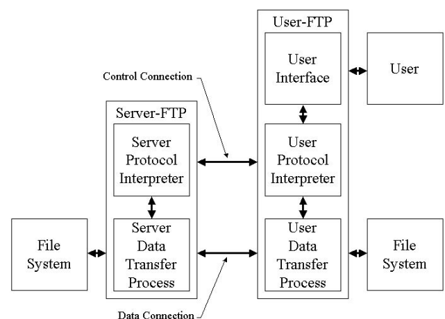
Fig -1: Normal Way-Data Transfer System
