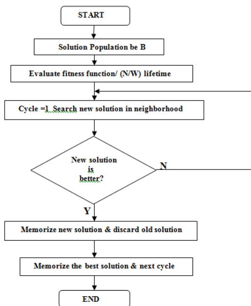
Fig 2. Flowchart for ABC Deployment
