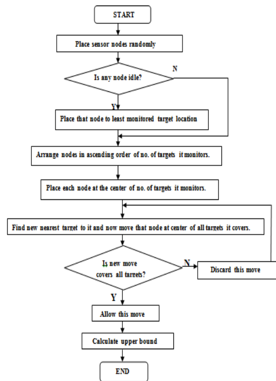
Fig.1 Flowchart for Heuristic Deployment
