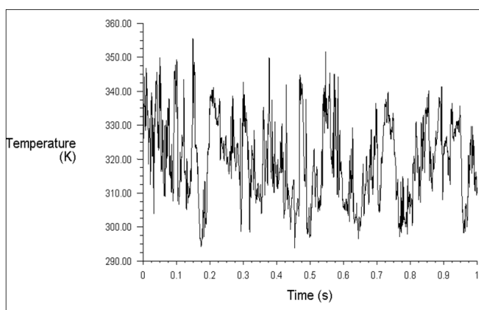
Chart 4.1: Temperature fluctuations of triangular nozzle
