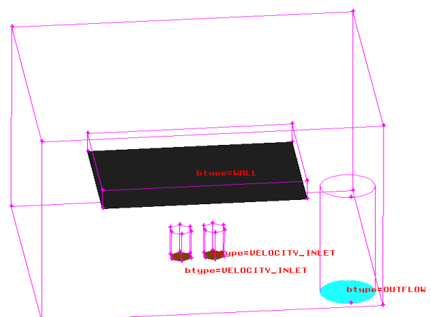
Fig 3.3: Hexagonal nozzle domain with boundary conditions
