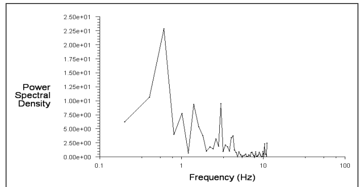
Chart 4.7: Power spectral density curve of triangular nozzle (Experiment)
