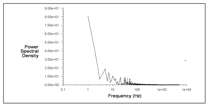
Chart 4.8: Power spectral density curve of triangular nozzle (Simulation)
