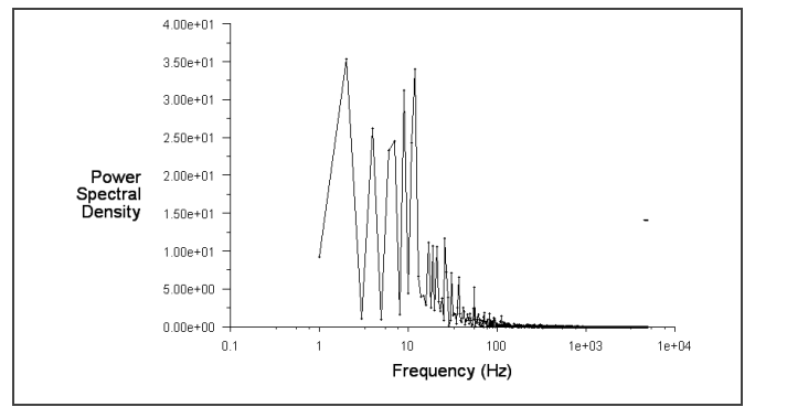
Chart 4.10: Power spectral density curve of hexagonal nozzle (Simulation)
