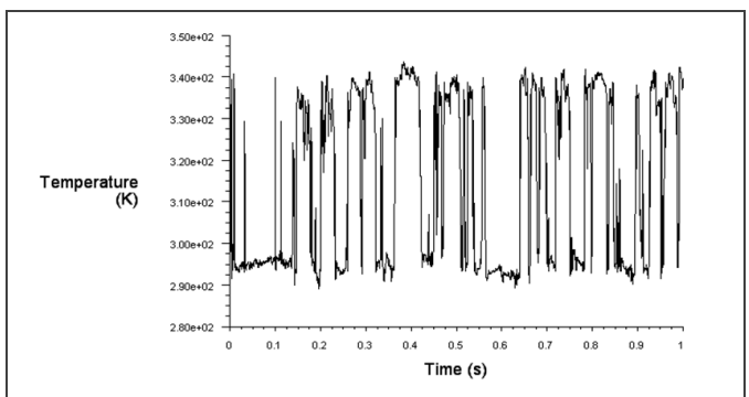
Chart 4.6: Temperature fluctuations of hexagonal nozzle (Simulation)
