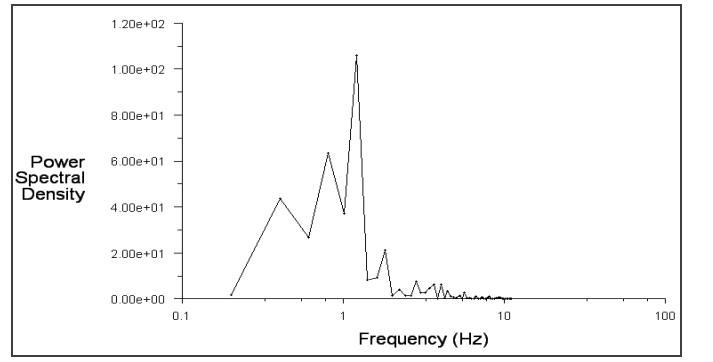
Chart 4.9: Power spectral density curve of hexagonal nozzle (Experiment)
