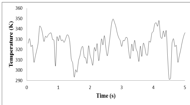
Chart 4.3: Temperature fluctuations of triangular nozzle (Experiment)
