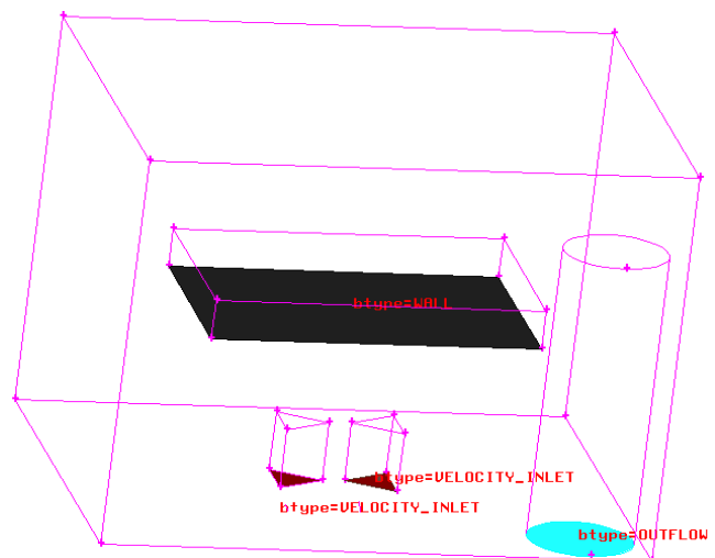
Fig 3.2: Triangular nozzle domain with boundary conditions
