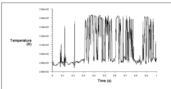
Chart 4.4: Temperature fluctuations of triangular nozzle (Simulation)
