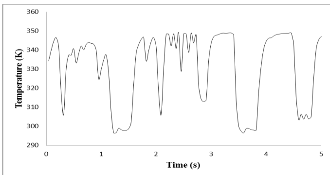
Chart 4.5: Temperature fluctuations of hexagonal nozzle (Experiment)
