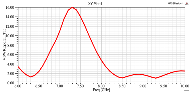
Figure4. Measured VSWR values at distinct frequency points
