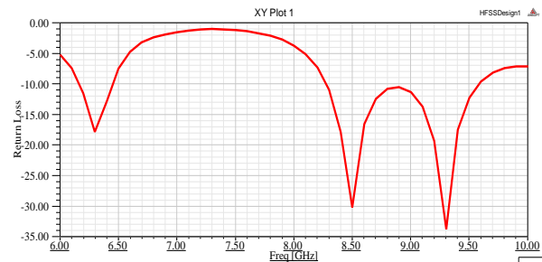
Figure3. Return Loss Vs frequency of designed antenna
