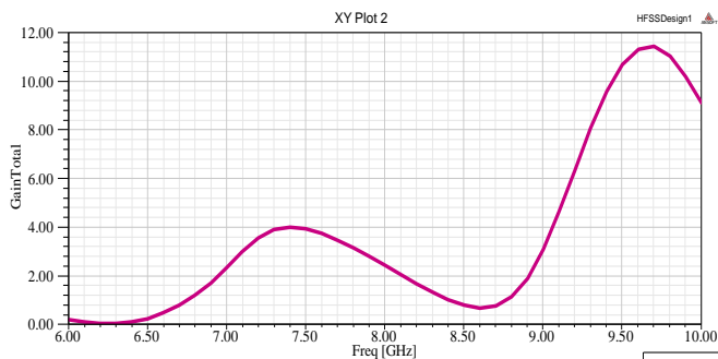
Figure5. Gain Vs frequency of designed antenna
