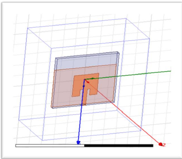
Figure2. Proposed antenna with defected ground structure (upside down view)
