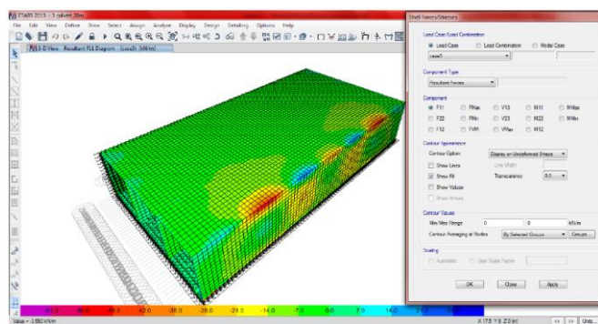
Fig.-10 Shell Member forces and Stress Diagram
