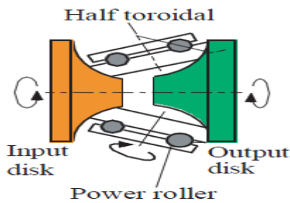
Fig.1 Toroidal type CVT
