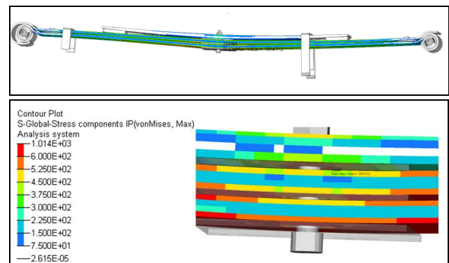
Fig.5: Contour Plot for leaf spring
