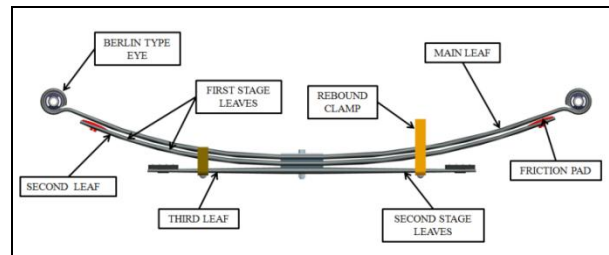
Fig.3 Leaf Spring nomenclature
