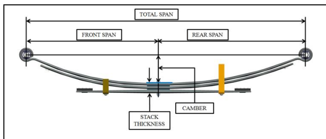
Fig.2 Leaf Spring parameters
