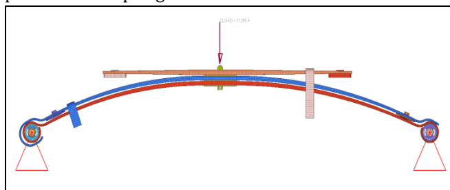
Fig.4: Boundary Condition
