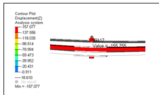
Fig.6: Displacement plot
