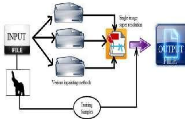
Fig 2. System architecture
