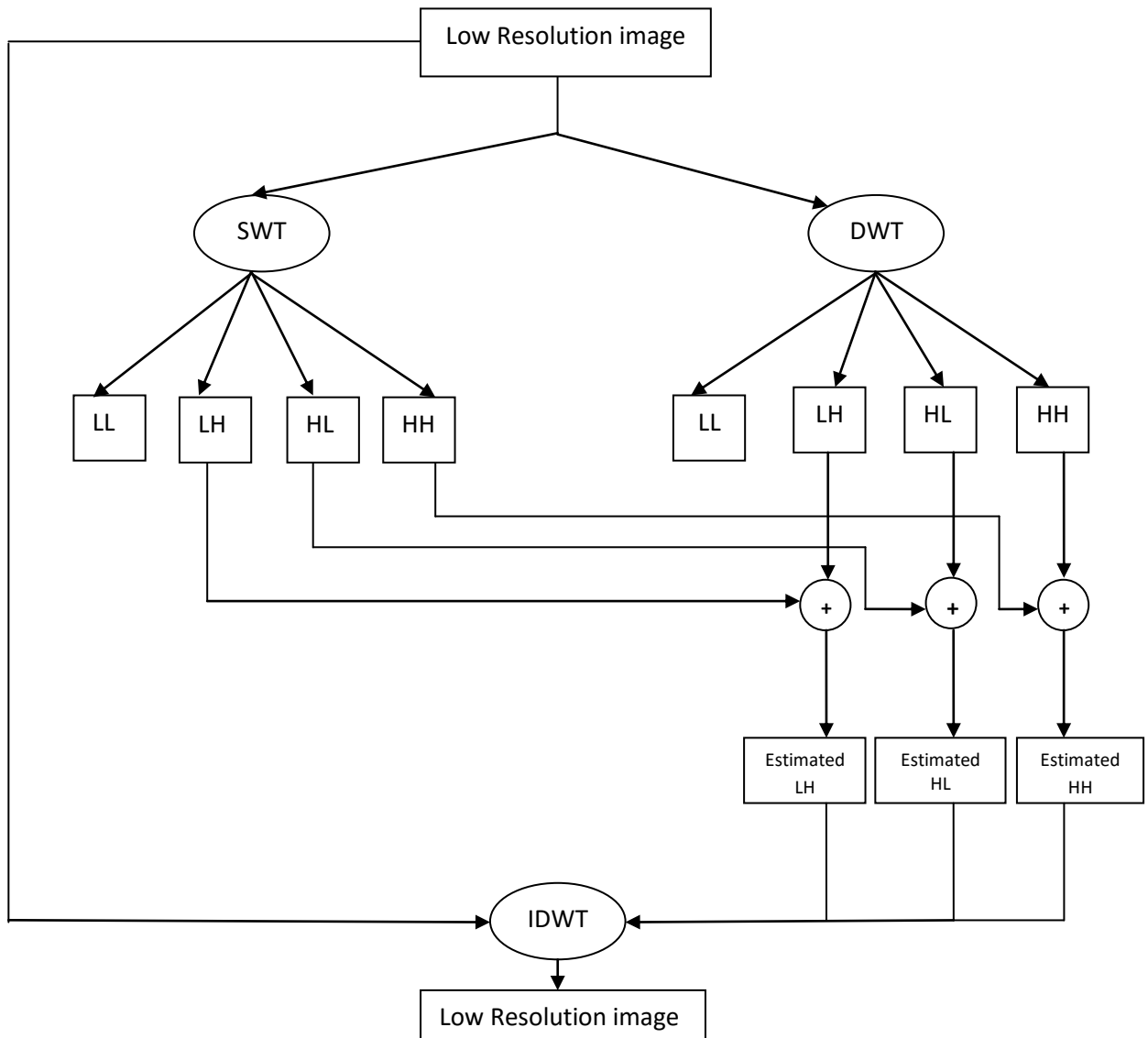
Fig.1. Block diagram of enhancement technique
