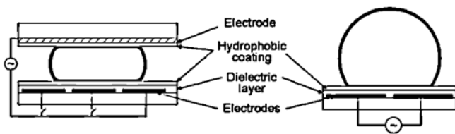
Fig -4: Schematics of closed and open Configuration of droplet microfluidic devices. In the open format, actuation and ground electrodes are housed in the bottom substrate
