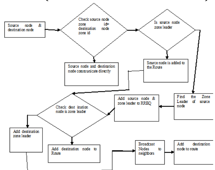
Fig.2: EBRP Routing Algorithm
