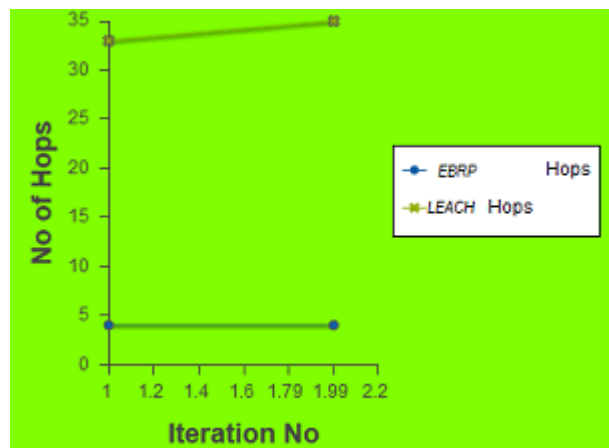
Chart2: Hops Comparison
