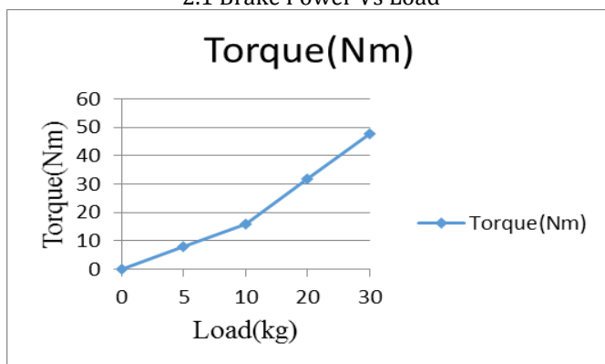
2.2 Torque Vs Load
