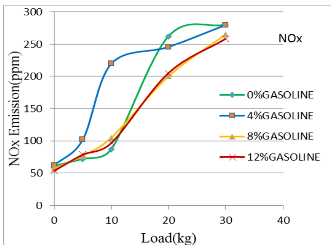
2.5 NOx Emission Vs Load
