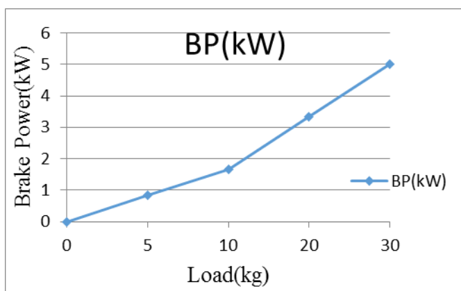
2.1 Brake Power Vs Load
