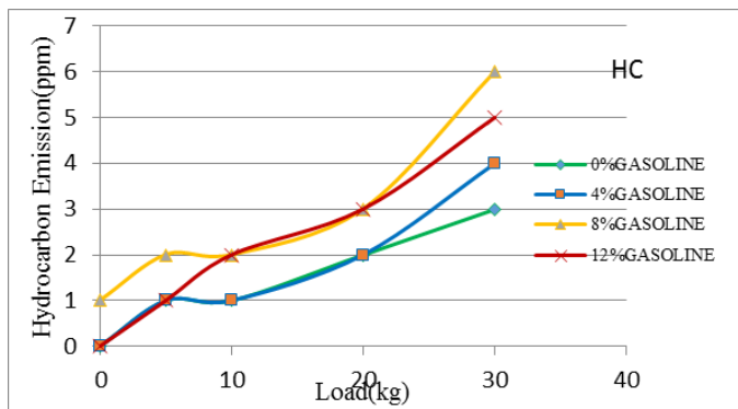
2.4 Hydrocarbon emission Vs Load
