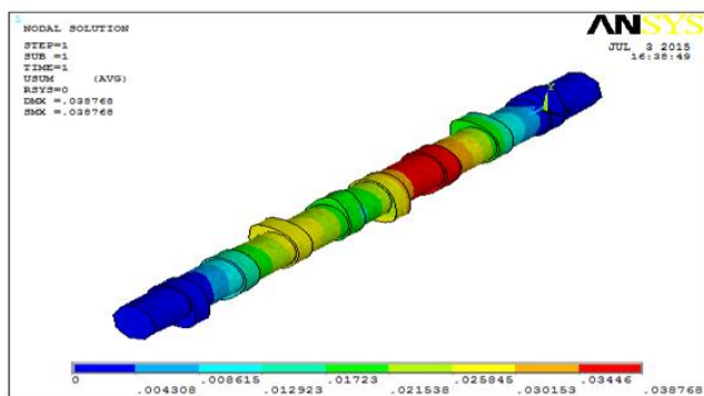
Fig -6: Displacement of cam
