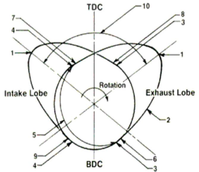
Fig -2: Cam specifications
