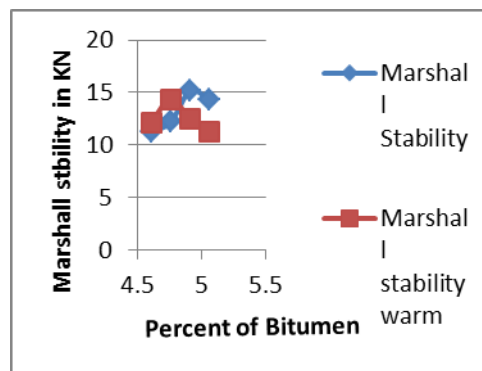
Fig 4.4.6 (g) Graphs of variation Marshall stability of warm mixes v/s hot mixes
