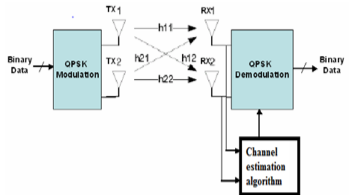
Fig-2: Block diagram of project
