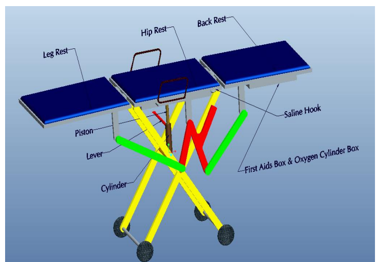
Fig 2.1 trolley-cum-wheelchair
