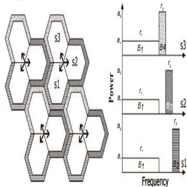
Figure 2: Fractional Frequency Reuse with Full Isolation (FFR-FI)
