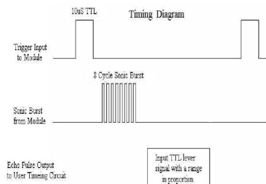
Fig 4: timing diagram for ultrasonic sensor
