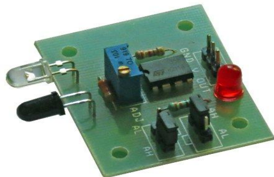
Fig1: IR sensor with transmitter and receiver
