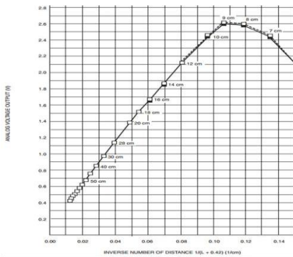
Fig 2: distance vs analogy output voltage
