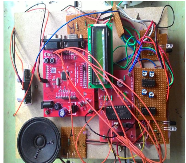
Fig 6: collision prediction using sensor system
