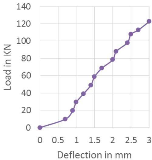
Natural Aggregate Beam
