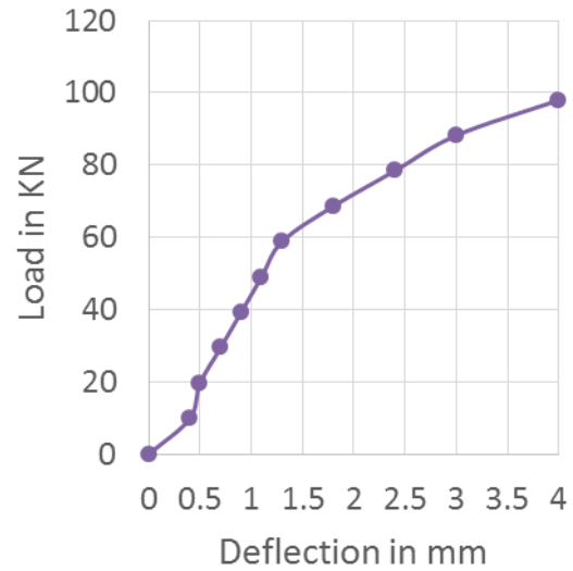
Treated Recycled Aggregate Beam
