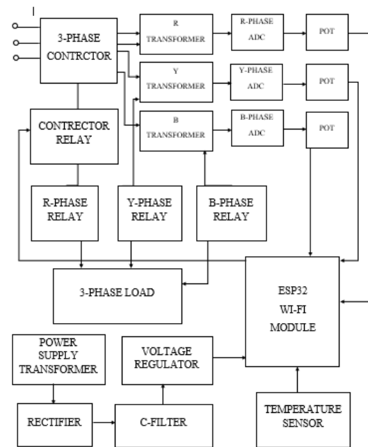
Fig.1: Block diagram
