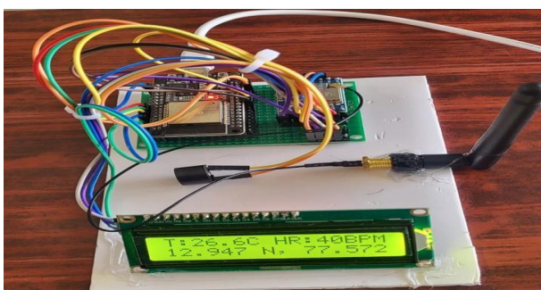
Fig.4.2 Base Station Setup for Soldier Monitoring and LoRa Communication.
