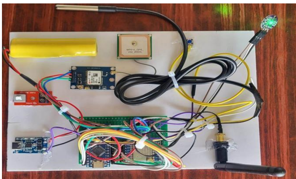
Fig.4.1. Hardware Integration of Proposed Soldier Monitoring System.
