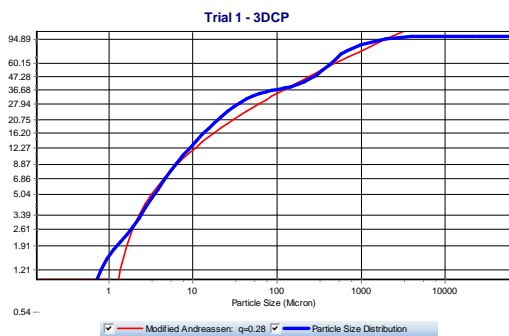
Fig -17: Output from EMMA - Particle size distribution of proposed mix (Blue colour) and Particle size distribution as per modified Andreassen model (Red colour)
