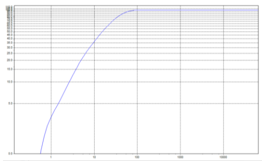
Fig -15: Particle size distribution curve for cement
