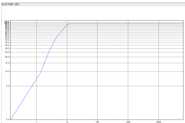
Fig -36: Particle size distribution curve for Alccofine
