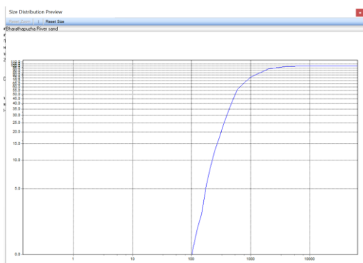
Fig -14: Particle size distribution curve for Bharatha puzha river sand
