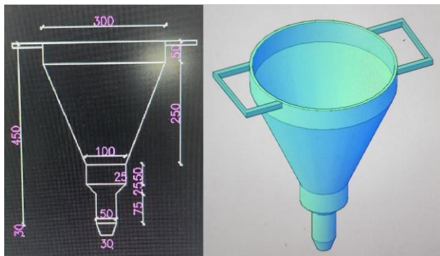
Fig -10: Concrete extruder for hand 3D printing: Conceptual drawing
