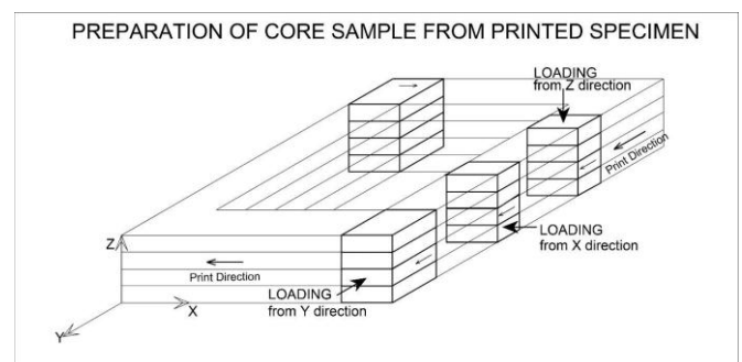
Fig -26: Diagram showing specimen preparation
