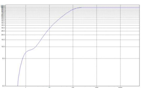
Fig -16: Particle size distribution curve for fly ash
