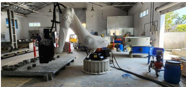
Fig -6: TVASTA's robotic arm printer at TVASTA Factory at OMR – Chennai. Accelerator dosing pump can be seen on right side.
