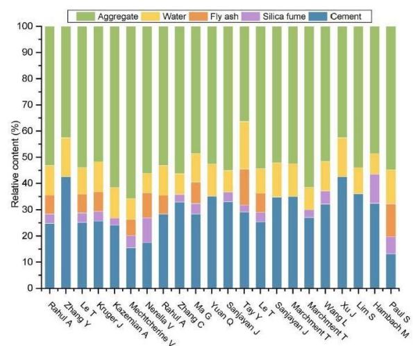
Fig -13: Relative content of binder, fly ash, silica fume, water, and aggregate in the optimum mixture proportion of 3DPCs
