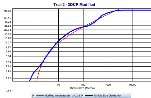
Fig -38: Particle size distribution of proposed modified green mix - Trial 02 (Blue colour) and Particle size distribution as per modified Andraessen (Red colour)
