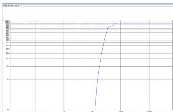
Fig -37: Particle size distribution curve for Rise husk ash
