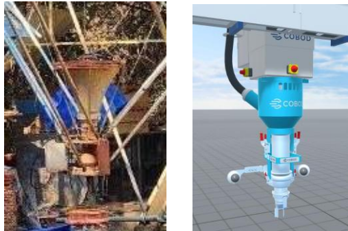
Fig -9: Extruder concept of Minvayu (Left) & COBOD (Right)
